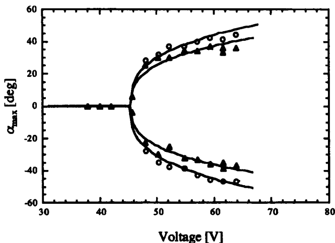
FIGURE 4 The in-plane rotation angle \alpha_{\max}(V) measured by gradually increasing (open circles) and suddenly raised (solid triangles) voltages (at f = 2150\text{Hz} ).
