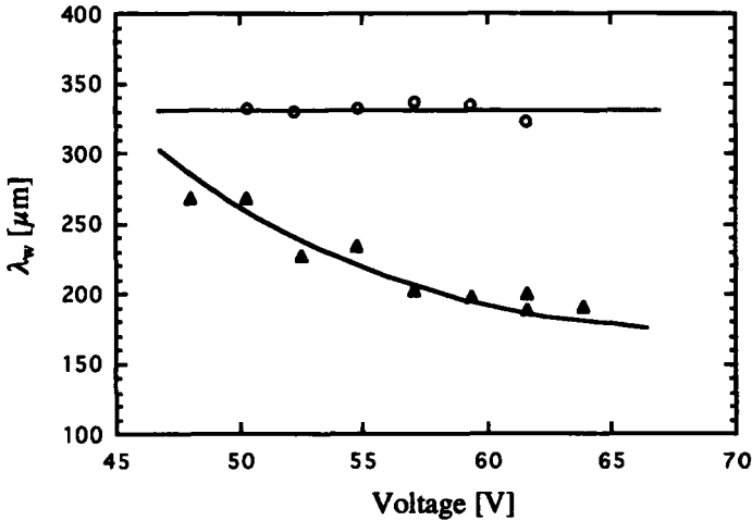
FIGURE 5 The wavelength \lambda_w of the prewavy pattern measured by gradually increasing (open circles) and suddenly raised (solid triangles) voltages (at f = 2150\text{Hz} ). The solid lines are to guide the reader's eye only.
